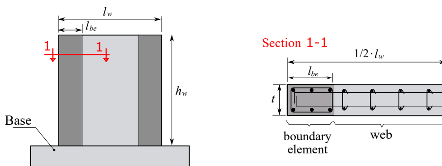
Figure 1: Components of a reinforced concrete shear wall and their corresponding notation.
