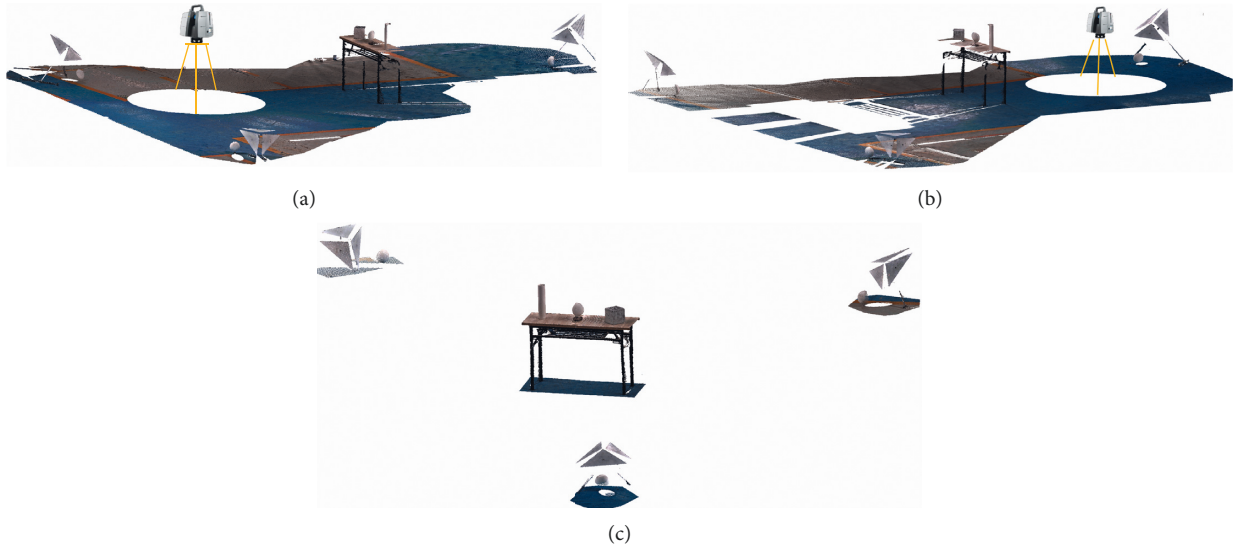
FIGURE 6: Scanning point cloud of verification experiment: (a) scanning point cloud 1, (b) scanning point cloud 2, and (c) point cloud after accurate registration.
