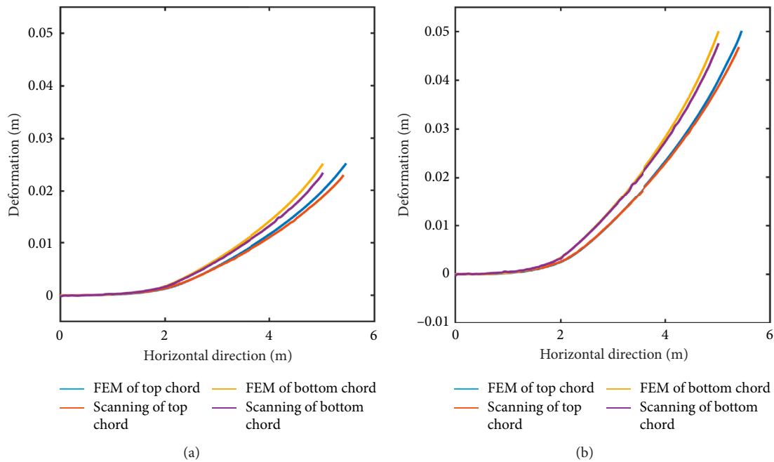
FIGURE 15: Deformation caused by forced displacement: (a) \delta = 2 mm and (b) \delta = 4 mm.
