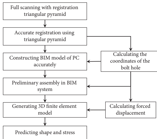
FIGURE 16: Proposed VTA process.
