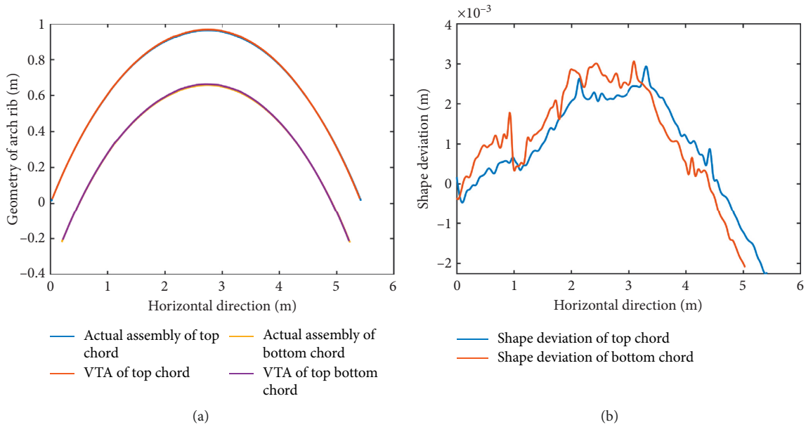
FIGURE 17: Results of the VTA for the experimental arch bridge: (a) geometry of the arch ribs and (b) geometric deviation.
