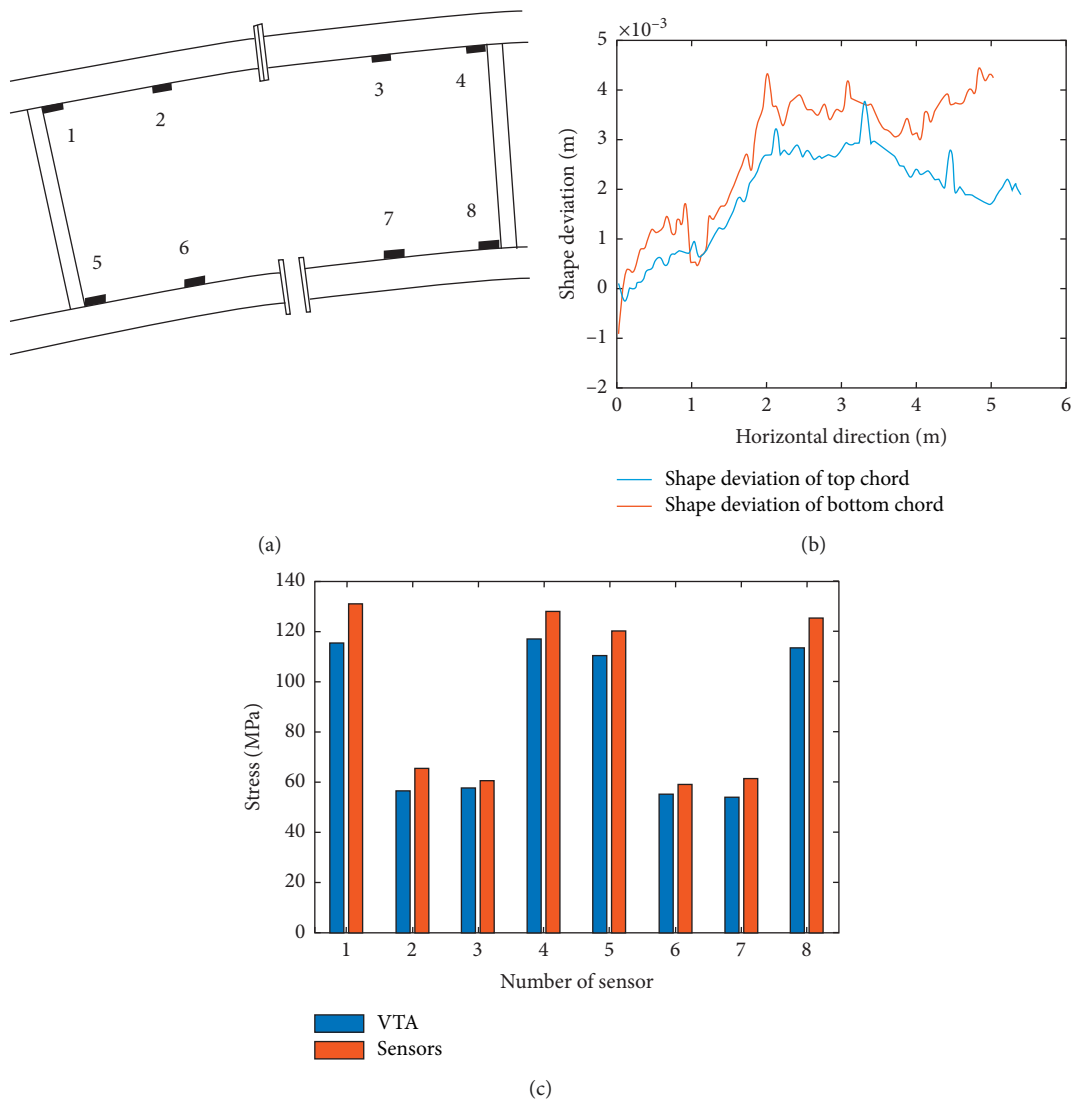
FIGURE 18: VTA experimental results ( \delta = 6 mm): (a) stress sensor arrangement, (b) geometric deviation, and (c) stress results.
