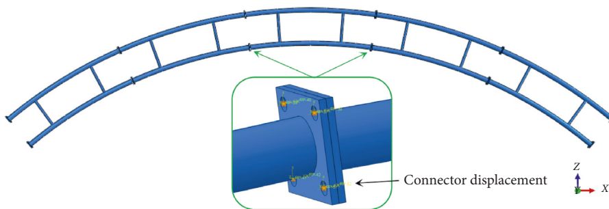
FIGURE 13: Finite element model of the experimental arch bridge.
