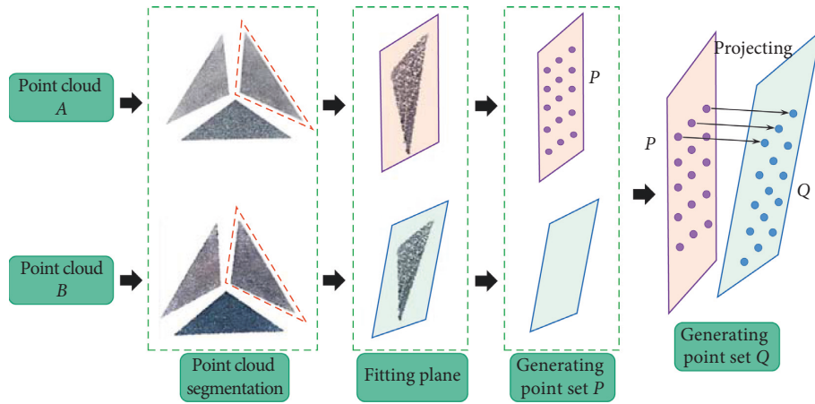
FIGURE 3: Precise registration process of a triangular pyramid marker.
