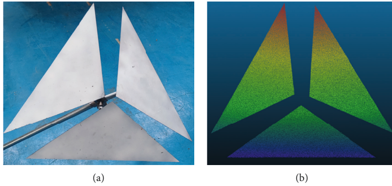
FIGURE 2: Triangular pyramid marker: (a) physical picture of a triangular pyramid marker and (b) point cloud of a triangular pyramid marker.
