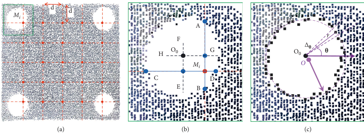
FIGURE 11: Example of the calculation process of the bolt hole center: (a) generate grid points, (b) calculate the circle center O_0 , and (c) calculate the circle center ( O ).
