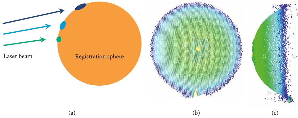
FIGURE 1: Edge drift of a spherical marker: (a) laser path of a registration sphere, (b) front view of a spherical point cloud, and (c) side view of a spherical point cloud.
