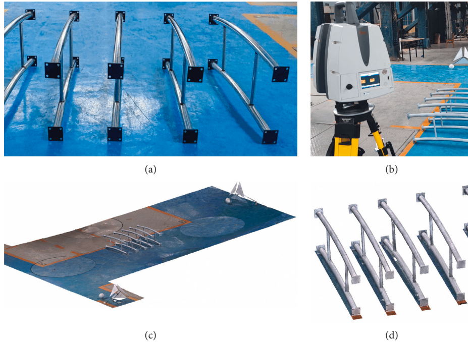
FIGURE 9: Scanning of the scaled arch bridge: (a) prefabricated segment, (b) on-site scanning, (c) registered point cloud, and (d) prefabricated segment point cloud segmentation.
