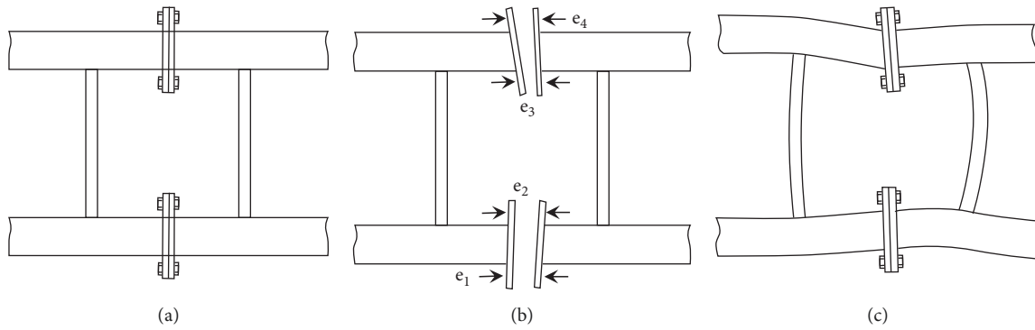
FIGURE 12: Bolt assembly process: (a) theoretical assembly, (b) assembly clearance, and (c) forced assembly.
