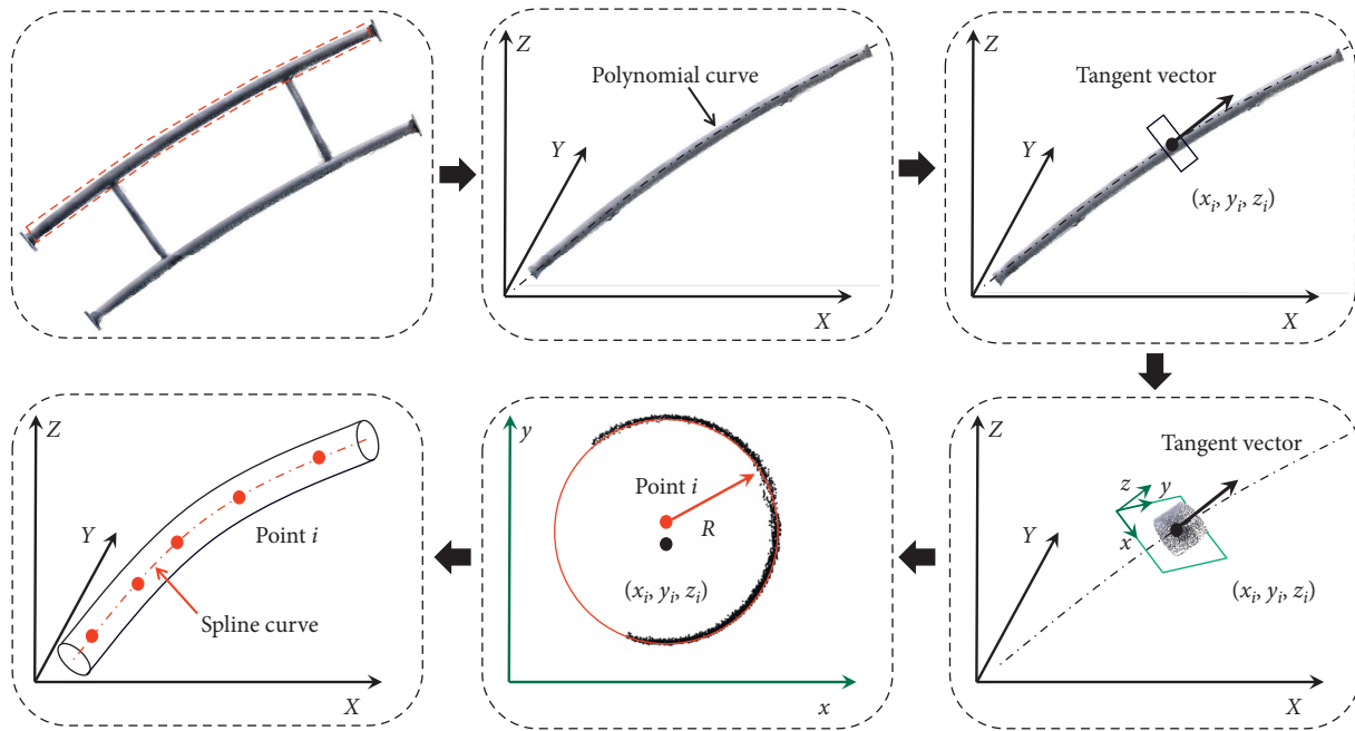
FIGURE 10: Reverse construction of the building information modeling steps of curved components.
