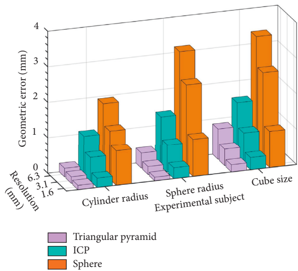
FIGURE 7: Geometric deviation of the experimental objects.
