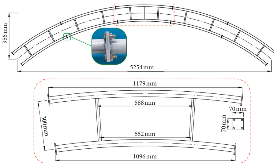
FIGURE 8: Design drawing of the scaled arch bridge.
