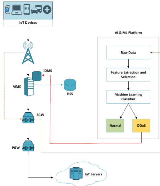
Figure 2: Proposed Method for Anomaly Detection
