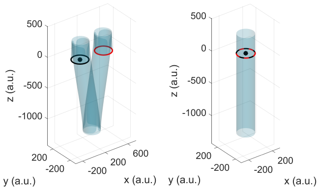
FIG. 2: Left panel: The classical translation of an initial circular Rydberg “state”, illustrated by a black ring, imposed by a two-cycle laser field of maximum electric field strength E_0 = 3 a.u. The black dot illustrates the position of the nucleus, whose influence is disregarded in this illustration. The red circle marks the resulting position. While the electric component imposes a strong excursion during interaction with the pulse, there is no net translation in the polarization direction ( z -axis) after the interaction. The radiation pressure, on the other hand, pushes the electron far into the propagation direction ( x -axis). Within the dipole approximation, there is no such push, and the initial and final positions coincide (right panel).
