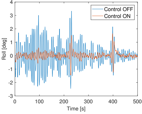
Fig. 5. Roll angle with and without cushion control, \psi = 135^\circ .
