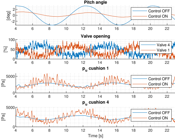
Fig. 3. Pitch angle, valve opening, cushion 1 pressure, cushion 4 pressure, for a T_p = 8s wave.
