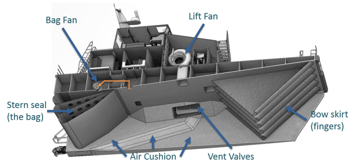
Fig. 1. Cross section of a SES. Illustration by Umoe Mandal.
