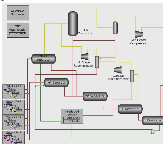
Fig.1 Overview of the large-scale oil and gas production plant model.
