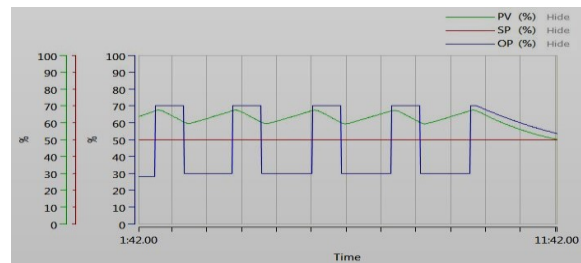
Fig.3 Level controller behavior during the simulation scenario.
