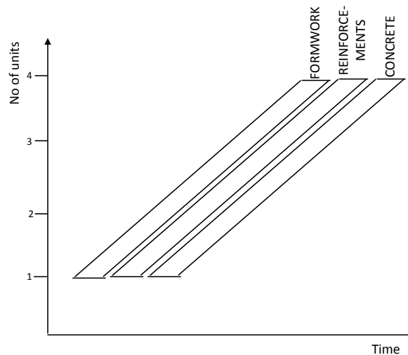
Figure 2. Illustration of a flowline chart
