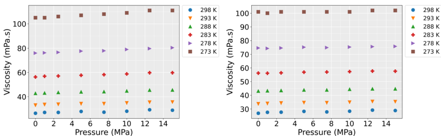
(a) viscosity vs pressure with varying temperatures at shear rate 300 \text{ s}^{-1} (b) viscosity vs pressure with varying temperatures at shear rate 1000 \text{ s}^{-1}
