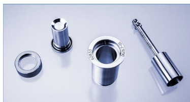
(b) High pressure set up in Double Gap geometry
