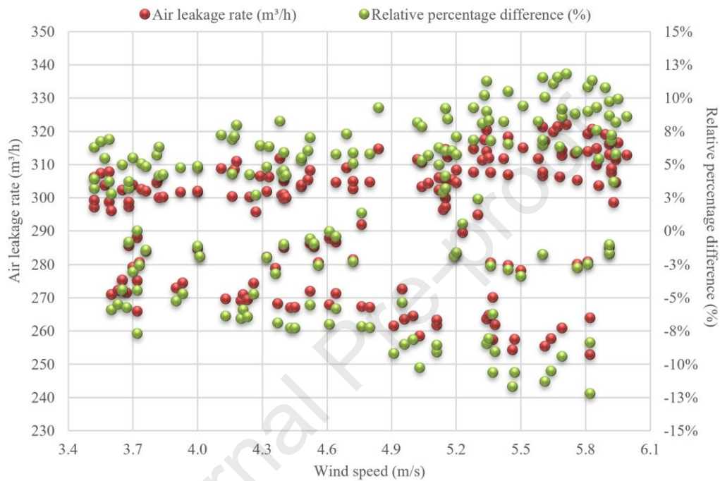
Figure 11: Test results in the wind speed range of 3.5-6m/s
