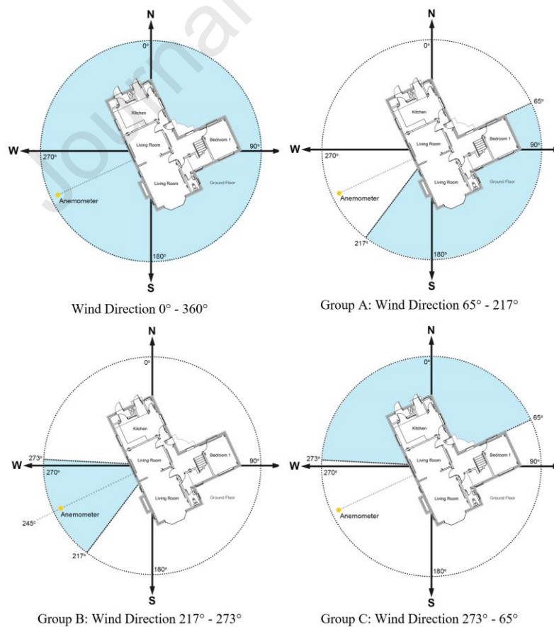
Figure 16: Illustration of different wind direction categories in relation to the test dwelling
