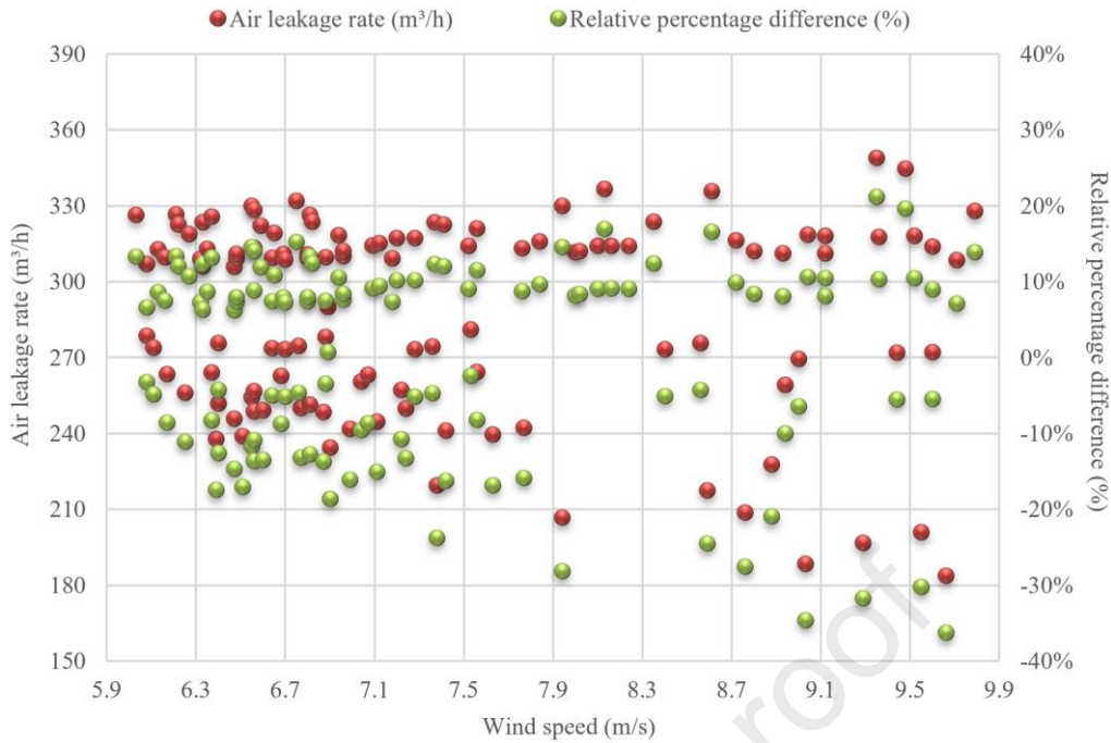
Figure 12: Tests results in the wind speed range of 6-10m/s
