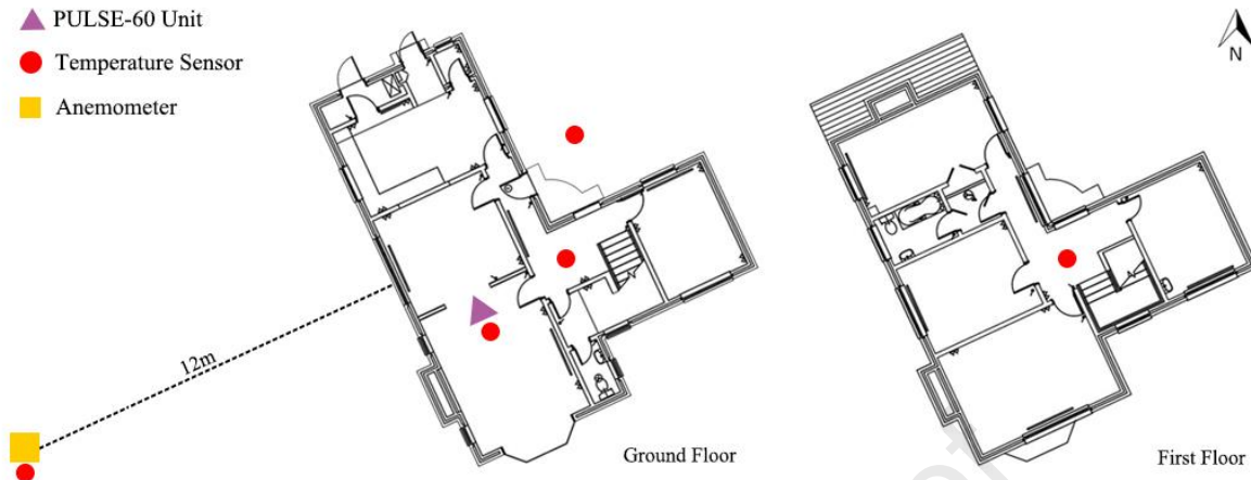
Figure 6: Illustration of the setup locations of test equipment
