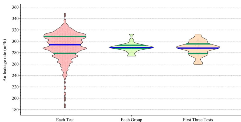
Figure 19: Violin plot of ALR results for the 423 tests, by each test, each group and first three tests
