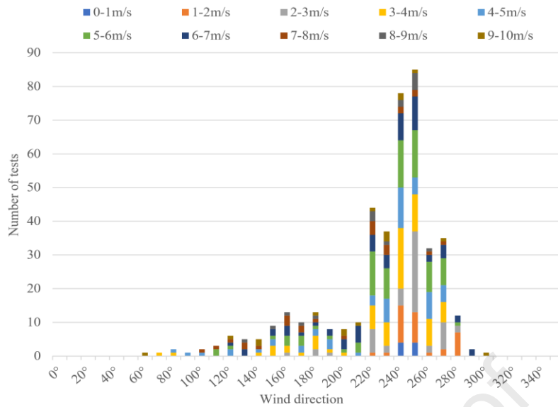
Figure 15: Wind direction distribution of 423 tests
