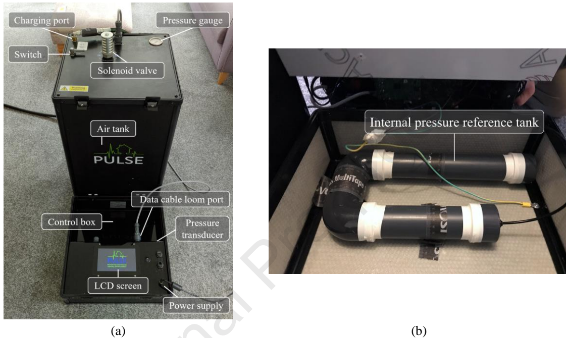
Figure 1: Photos of (a) PULSE-60 unit and (b) internal pressure reference tank of PULSE-60 unit
