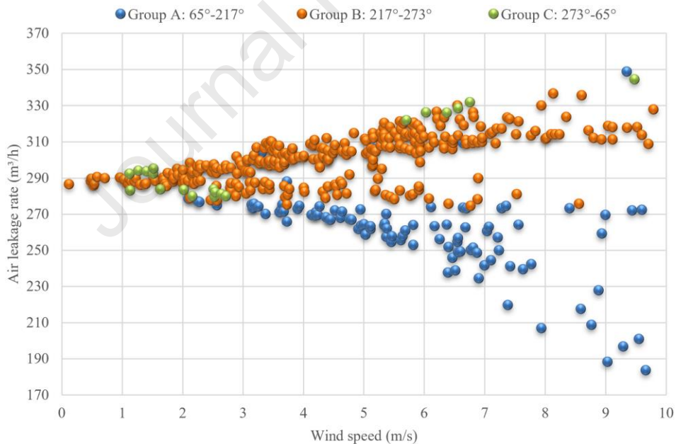
Figure 17: ALR measurements under different wind directions
