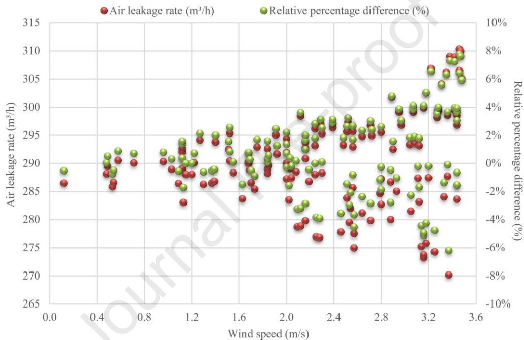
Figure 10: Test results in the wind speed range of 0-3.5m/s
