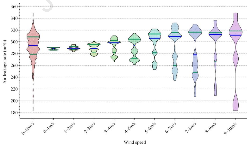
Figure 9: Violin plot of 423 tests
