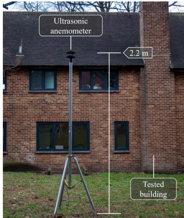
Figure 2: Photo of ultrasonic anemometer
