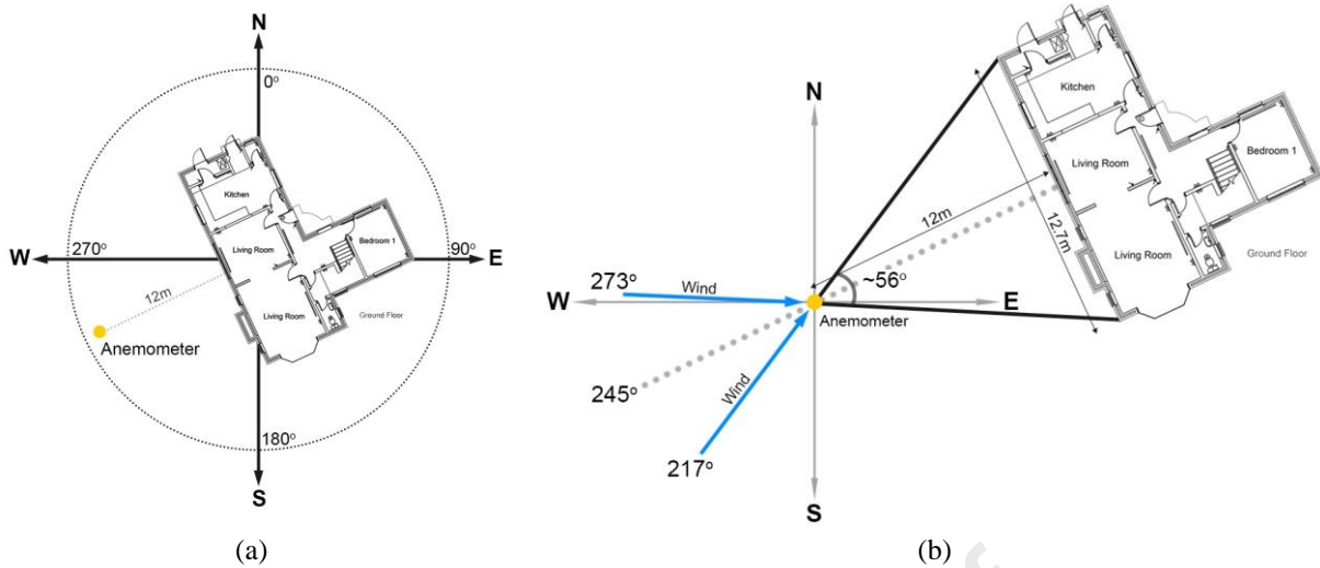
Figure 13: Illustrations of (a) test dwelling orientation and (b) anemometer orientation and wind directions with respect to test dwelling
