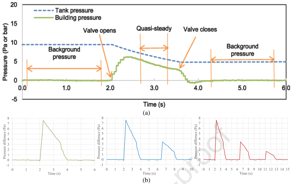
Figure 7: (a) Pressure variation with time for a typical Pulse test [12] and (b) pressure profiles during the one-step, two-step and three-step Pulse test
