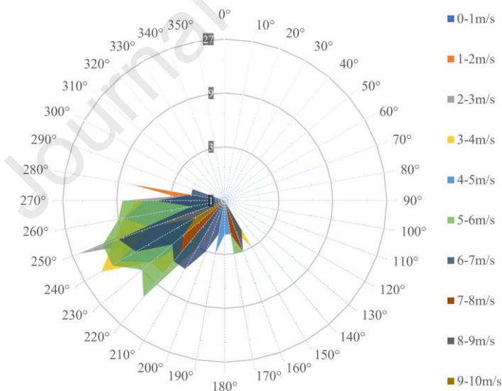
Figure 14: Wind rose plot of wind condition distribution of 423 tests
