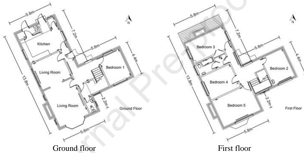
Figure 4: Building plans of the tested dwelling
