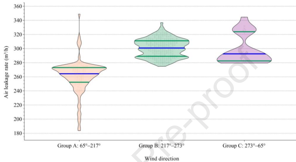
Figure 18: Violin plot of ALR results under different wind directions
