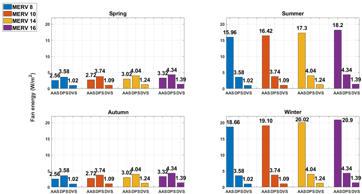
Figure 7. The fan loads of the three different ventilation strategies when equipped with the different grades of air filters for the four seasons.
