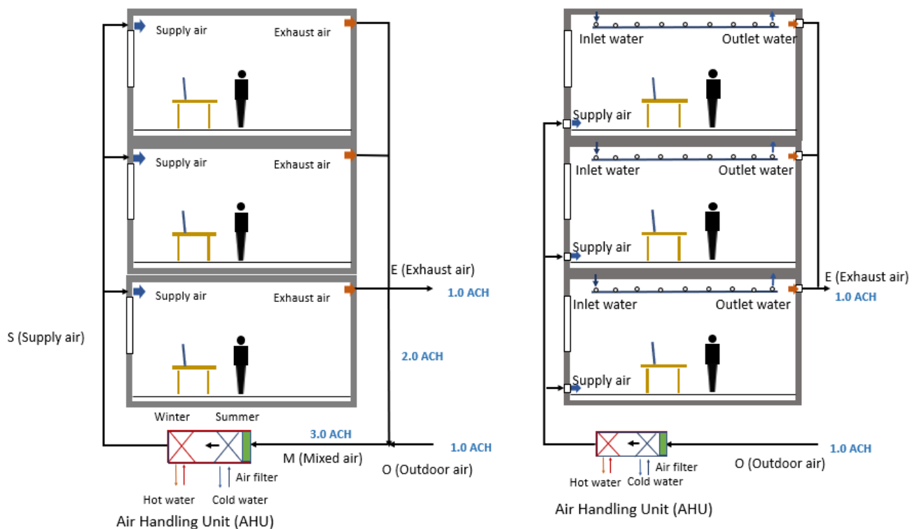
Figure 3. The installation of the ductwork in the building applied with a CV system.
