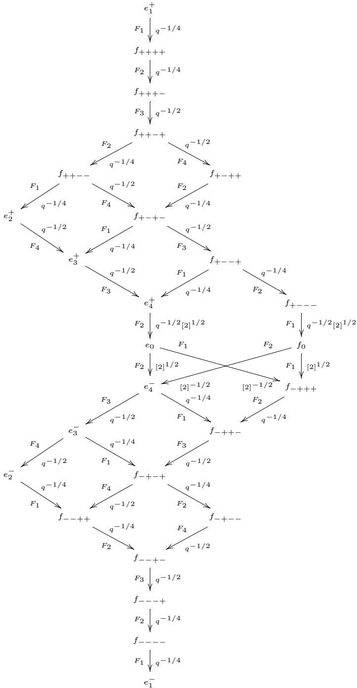
Diagram 1. Action of the F_r on V .
