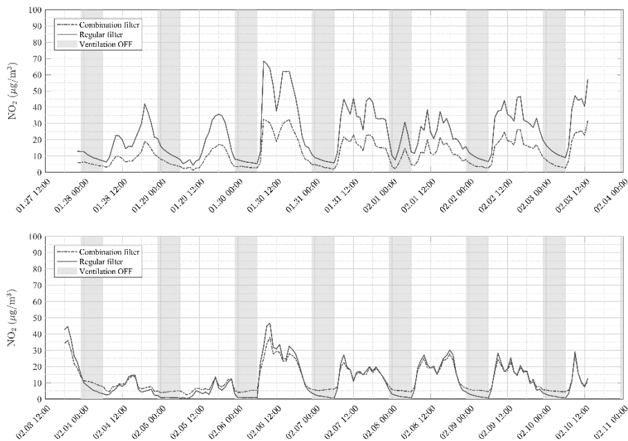
Fig. 3. \text{NO}_2 concentrations measured simultaneously inside two classrooms during sampling period 1 and 2. The filters in the ventilation systems of the two classrooms were switched between the measurement periods. Values are 1-h averages.
