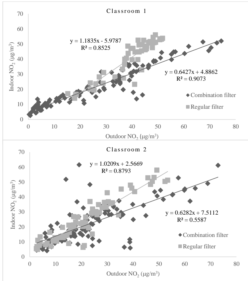
Fig. 4. Scatterplots of 1-h average (00-24 hours) NO 2 concentrations measured outdoor and indoor during sampling period 3-4 (upper) and 5-6 (lower).
