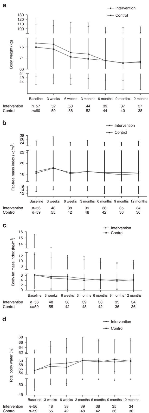
Fig. 2 Mean values and standard errors for: a body weight (kg), b fat-free mass index ( \text{kg}/\text{m}^2 ), c body fat mass index ( \text{kg}/\text{m}^2 ) and d total body water (%) during 1-year follow-up
