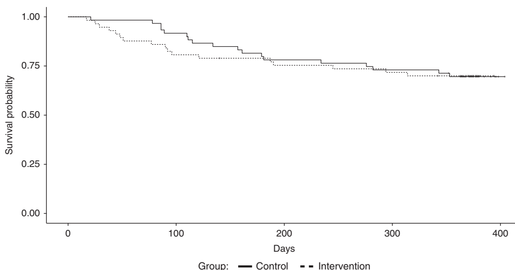
Fig. 1 Kaplan–Meier plot for 1-year overall survival
