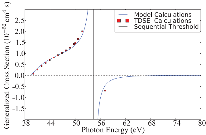
FIG. 4. (Color online) The first-order contribution to the total probability of double ionization, as obtained from the model—both under and over the sequential threshold. As in Fig. 1, the results have been given in units corresponding to a generalized cross section. The red points are results obtained from the full solutions of the TDSE. The TDSE results below threshold are taken from Ref. [12].
